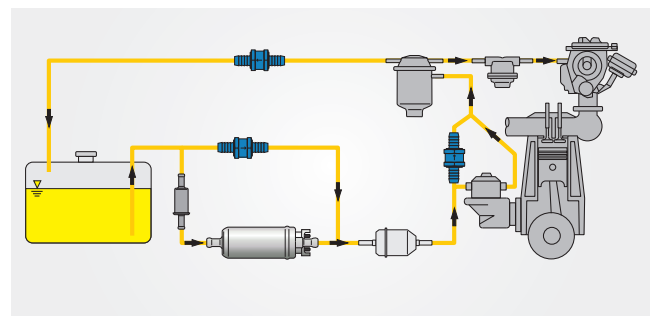
Application example: Carburettor engine with connectible supplementary electrical pump
