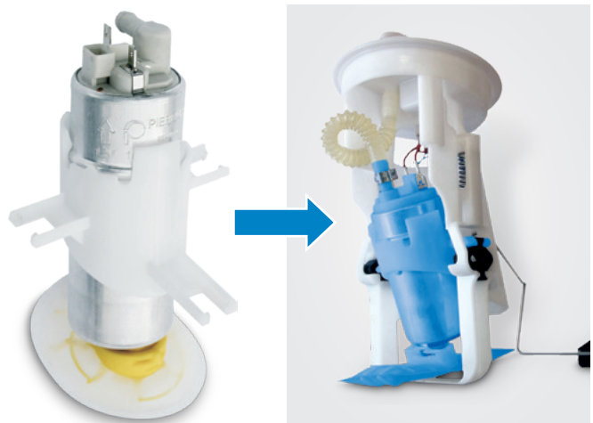
Spare parts set for fuel delivery module
